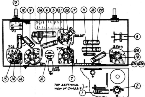
FIG. 1 — LOCATIONS OF PARTS — UNDERSIDE OF CHASSIS.
